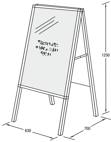
T-AS1 Equipped with 2 alternate frames
