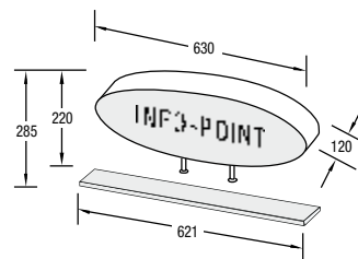
OT 120 Top plate, illuminated 16W/230V with inscription
