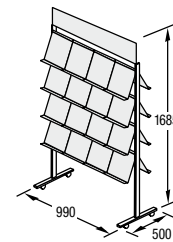
P-32T 32 shelves A4 + top plate
