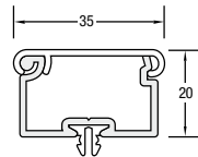
M 1485 Cable Way, aluminium
