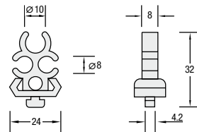
M 1488 Extrusion Clip plastic
