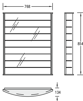
TM-Set 86 shelves 8 Outside dimensions: W 768 x H 854 x D 134 mm
