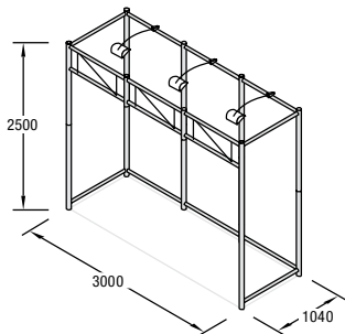
Q 20 Construction set including transport case Q 502 and lighting weight: 120.15 lb/54.5 kg
