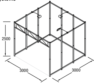
Q 40 Construction set including 2 transport cases Q 501, Q 502 and lighting weight: 176.37 lb/80.0 kg
