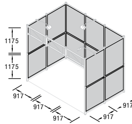
Q 32 Wall infill panel set "wood", white, 3.2 mm, including 7 beams and wooden case weight: 119.05 lb/54.0 kg
