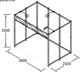
Q 30 Construction set including transport case Q 502 and lighting weight: 147.71 lb/67.0 kg
