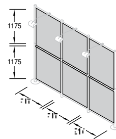
Q 12 Wall infill panel set "wood", white, 3.2 mm, including 3 beams and wooden case weight: 52.91 lb/24.0 kg
