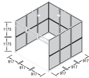
Q 42 Wall infill panel set "wood", white, 3.2 mm, including 9 beams and transport case Q 503 Suspending the fabric panel weight: 178.57 lb/81.0 kg
