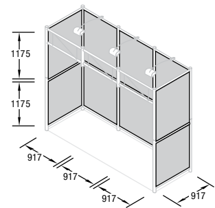
Q 22 Wall infill panel set "wood", white, 3.2 mm, including 5 beams and wooden case weight: 85.98 lb/39.0 kg
